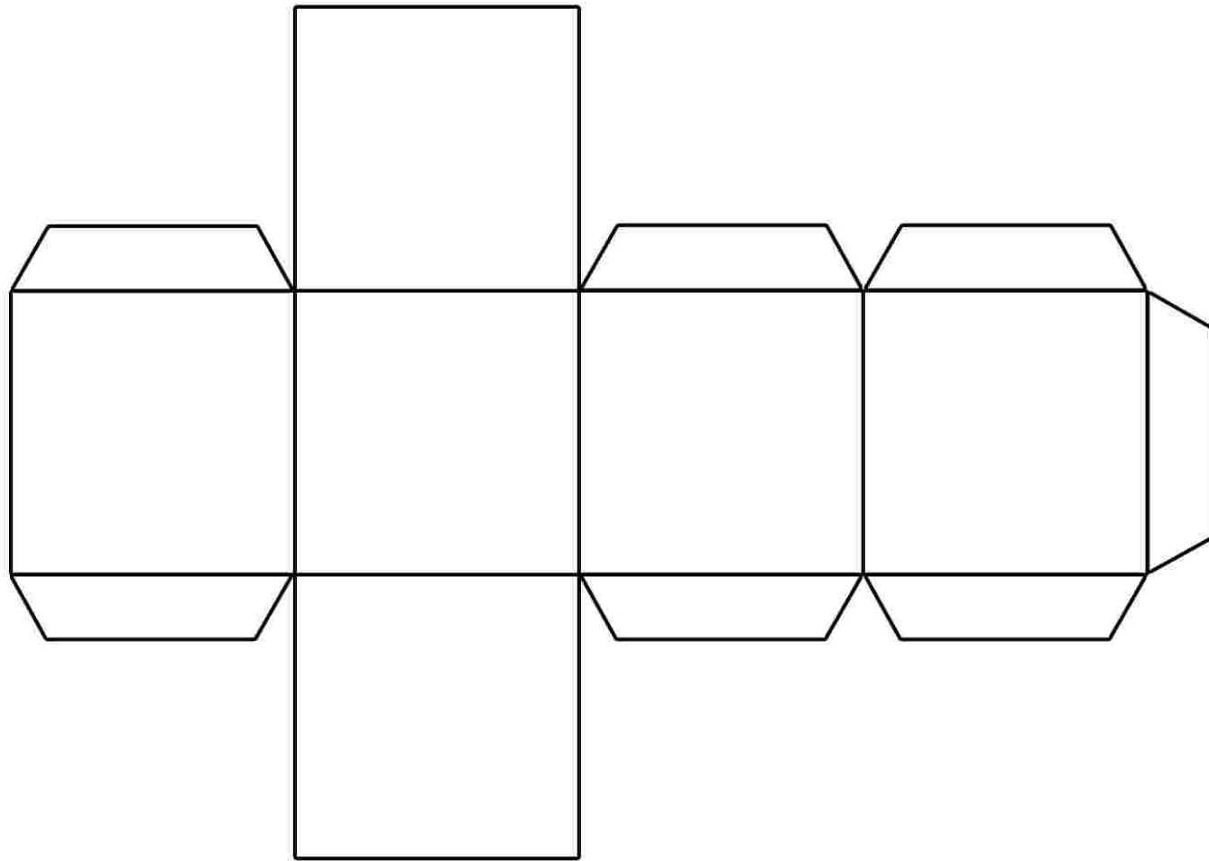
Hexahedron (platonic solid)
